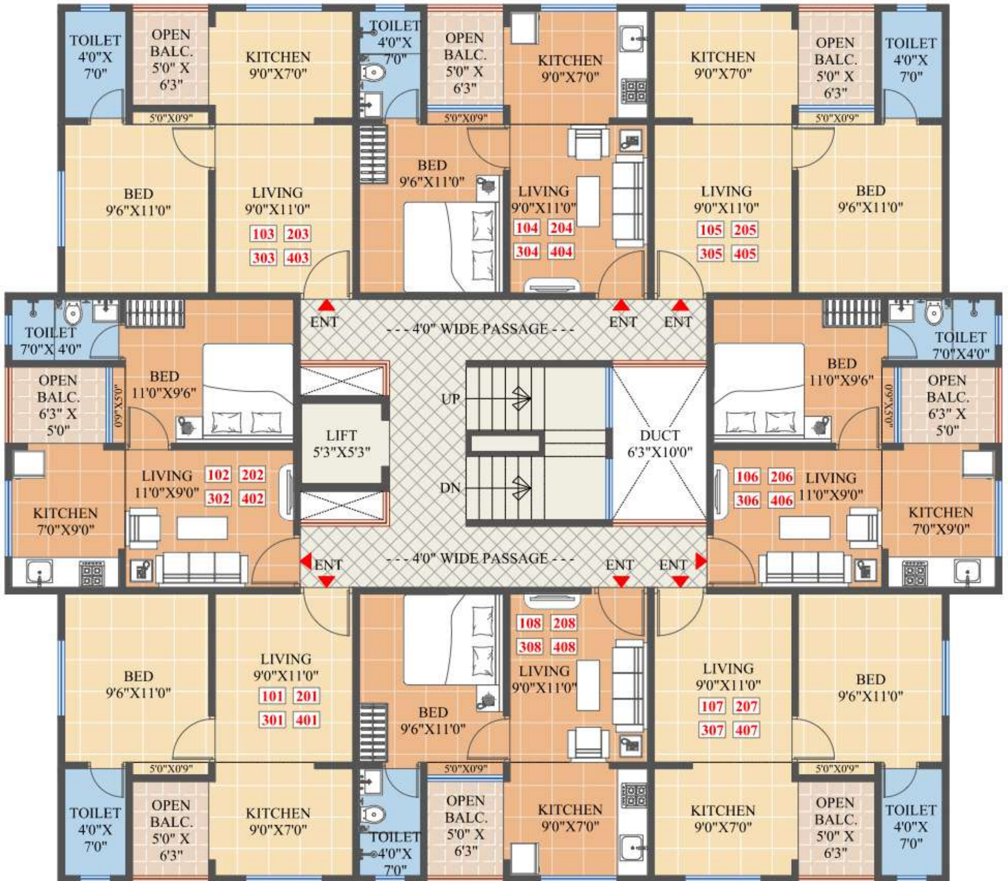
1ST,2ND,3RD,4TH FLOOR PLAN
