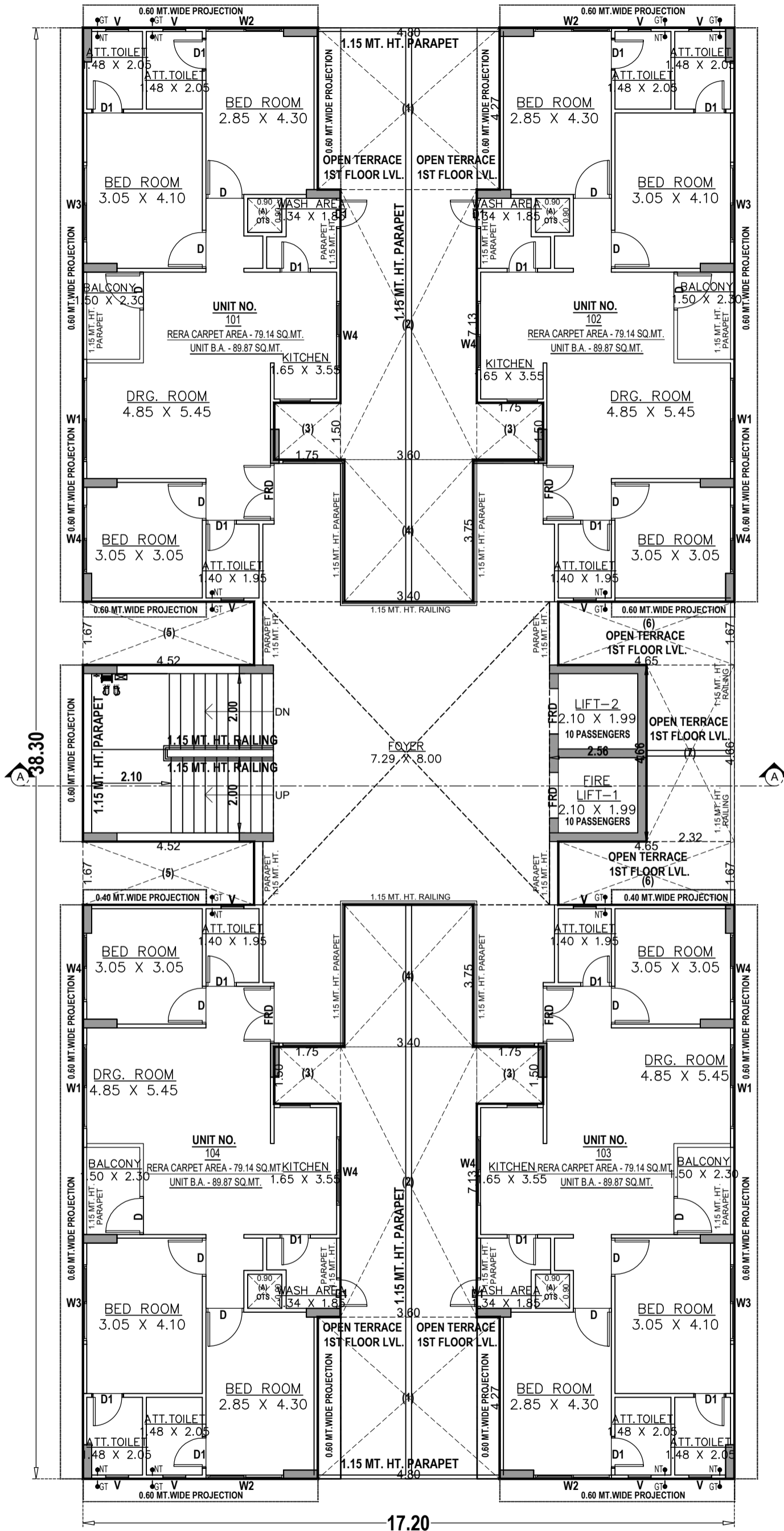
17.20 1ST FLOOR PLAN
