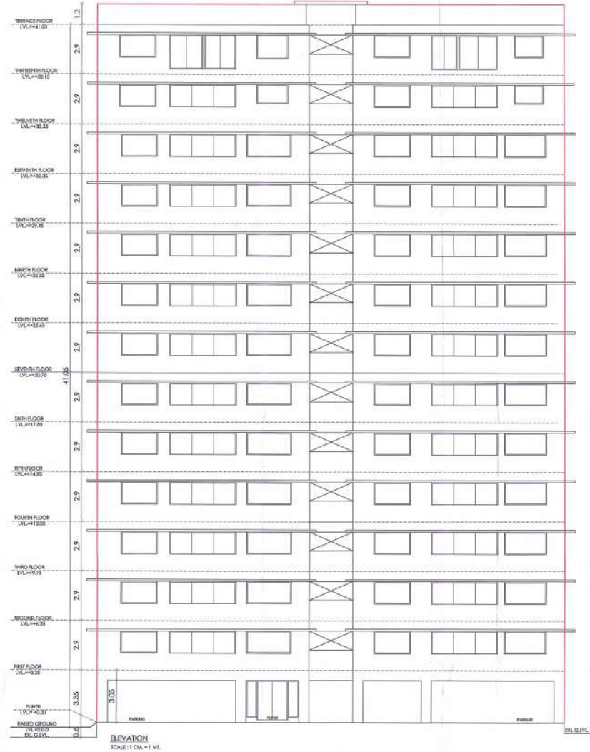
A&B Section Elevation Plan
