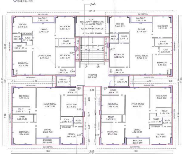
13th FLOOR PLAN SCALE: 1/8" = 1'-0"
