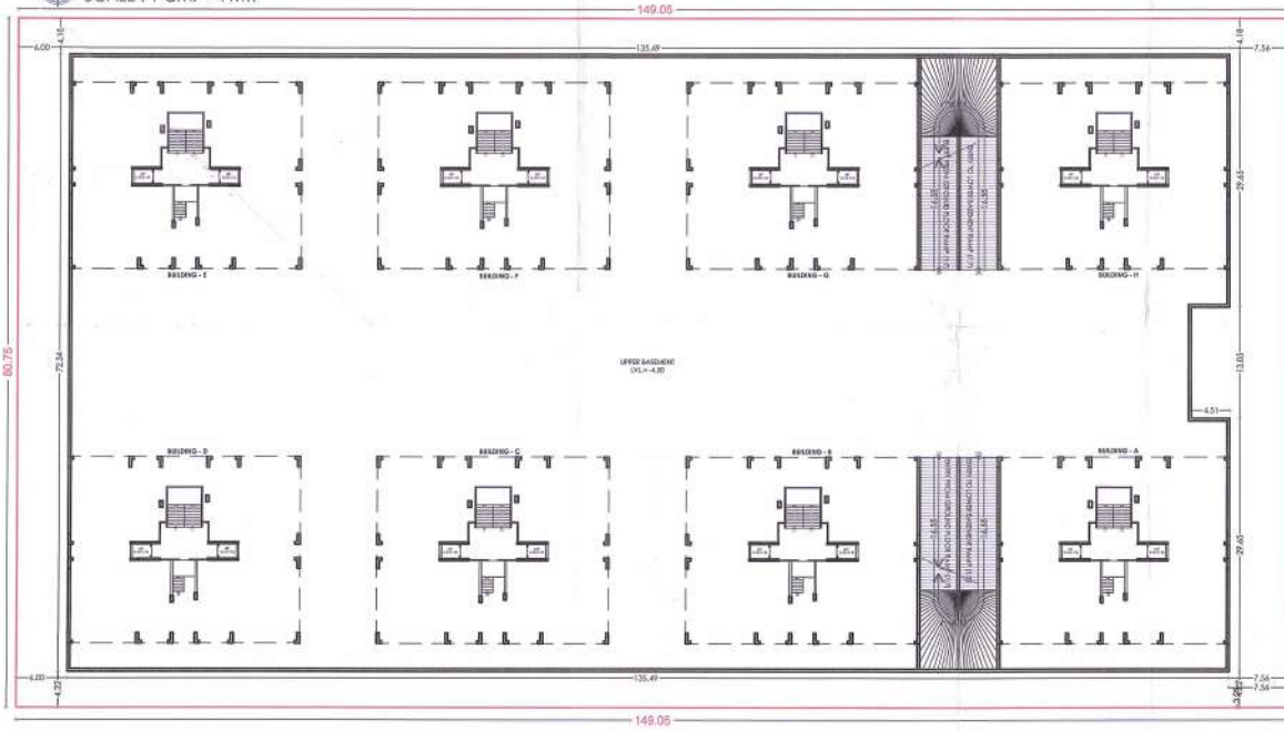
UPPER BASEMENT LAY-OUT PLAN SCALE : 1 CM. = 4 MT.
