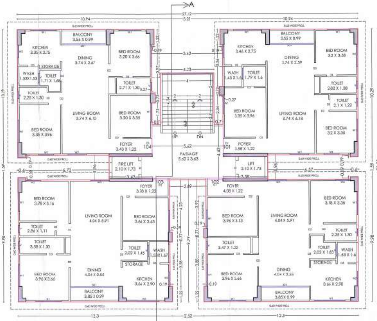
TYPICAL 1st TO 12th FLOOR PLAN SCALE: 1/8" = 1'-0"
