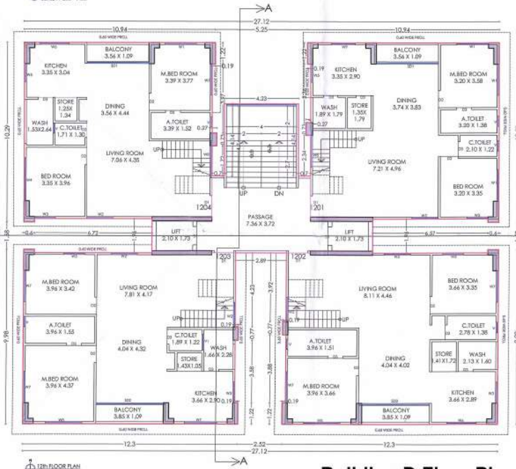
Building D Floor Plan
