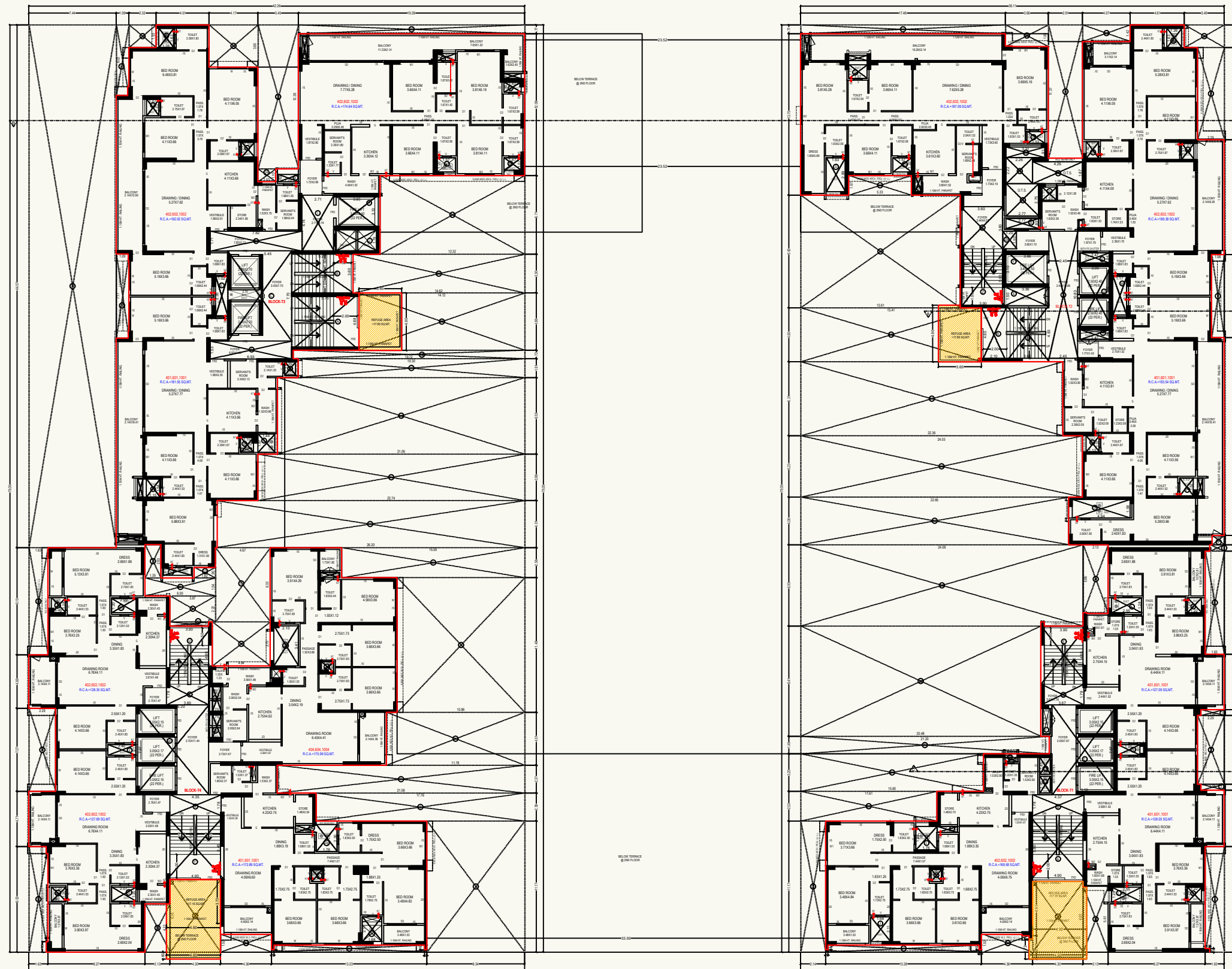
4TH, 6TH & 10TH FLOOR PLAN (REFUGE AREA FLOOR)
