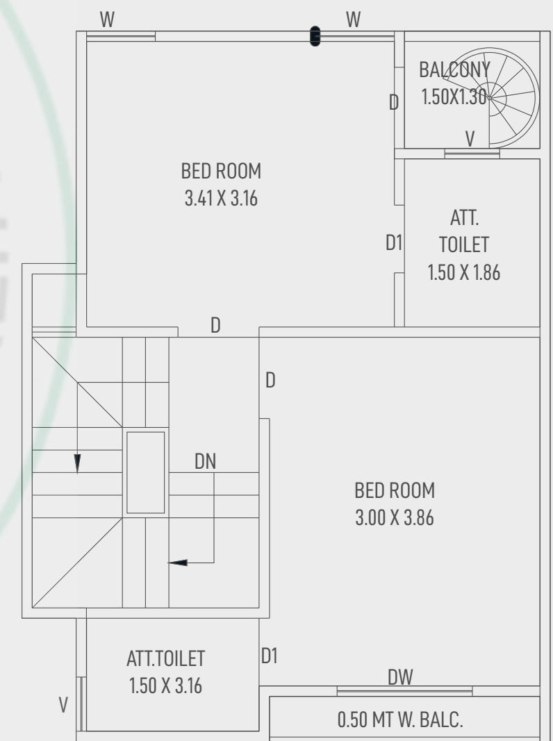
SECOND FLOOR PLAN (TYPE-D)
