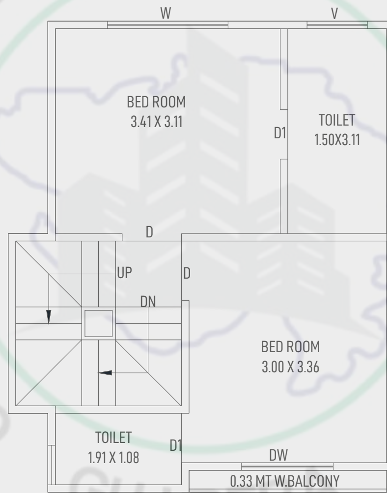
FIRST FLOOR PLAN (TYPE-B2)
