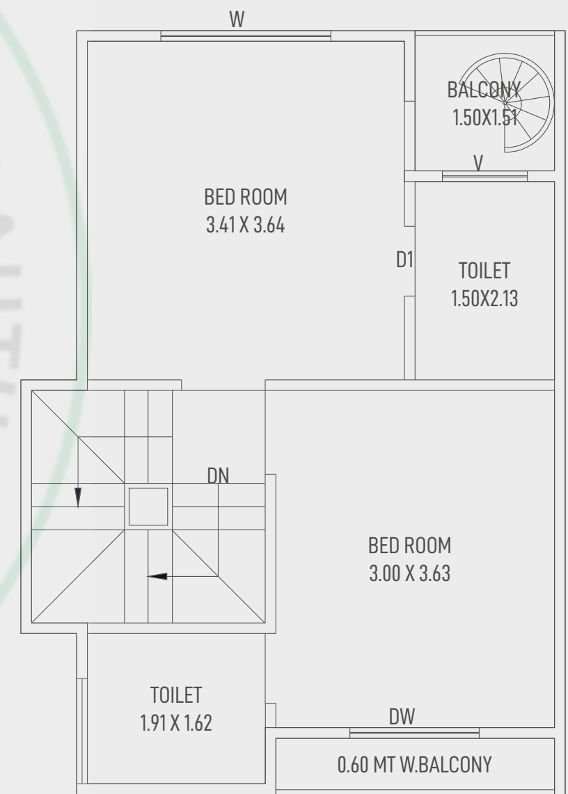
SECOND FLOOR PLAN (TYPE-B1)
