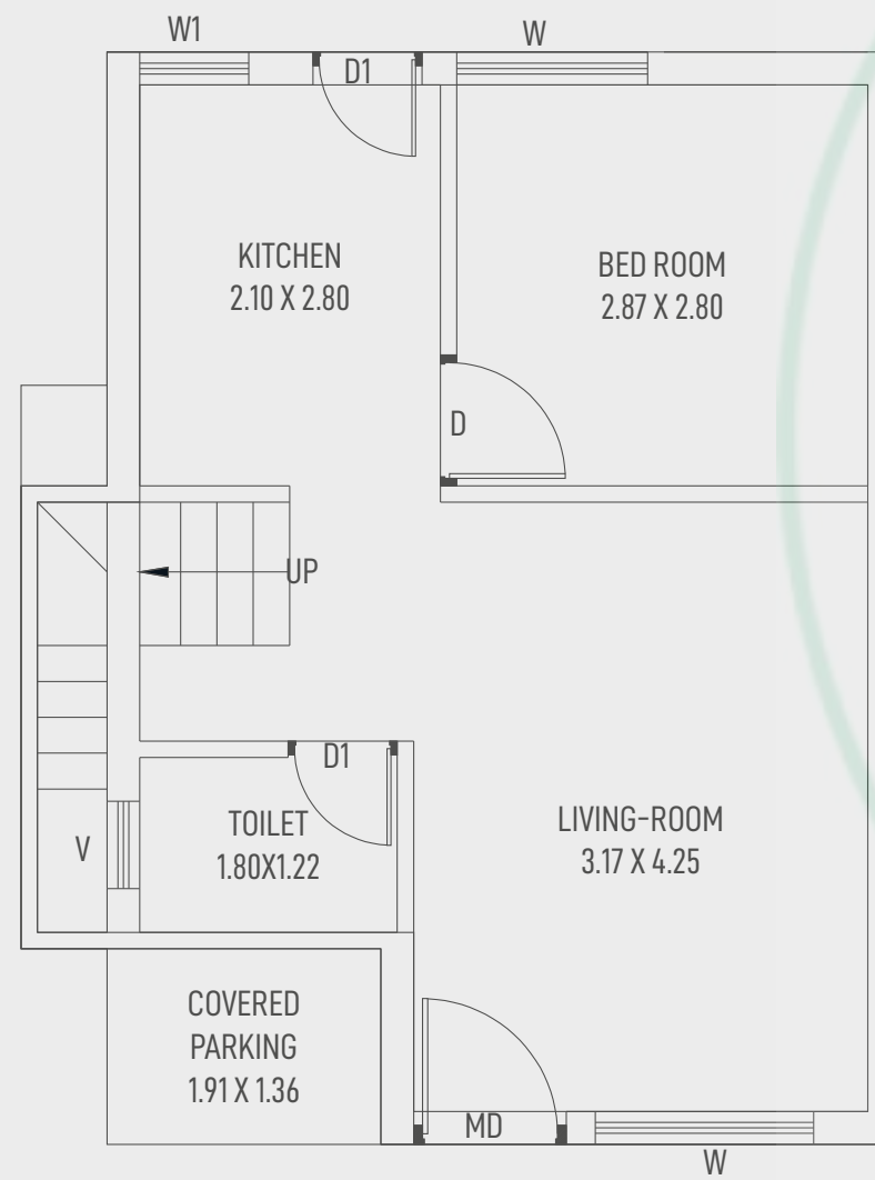
GROUND FLOOR PLAN (TYPE-A)
