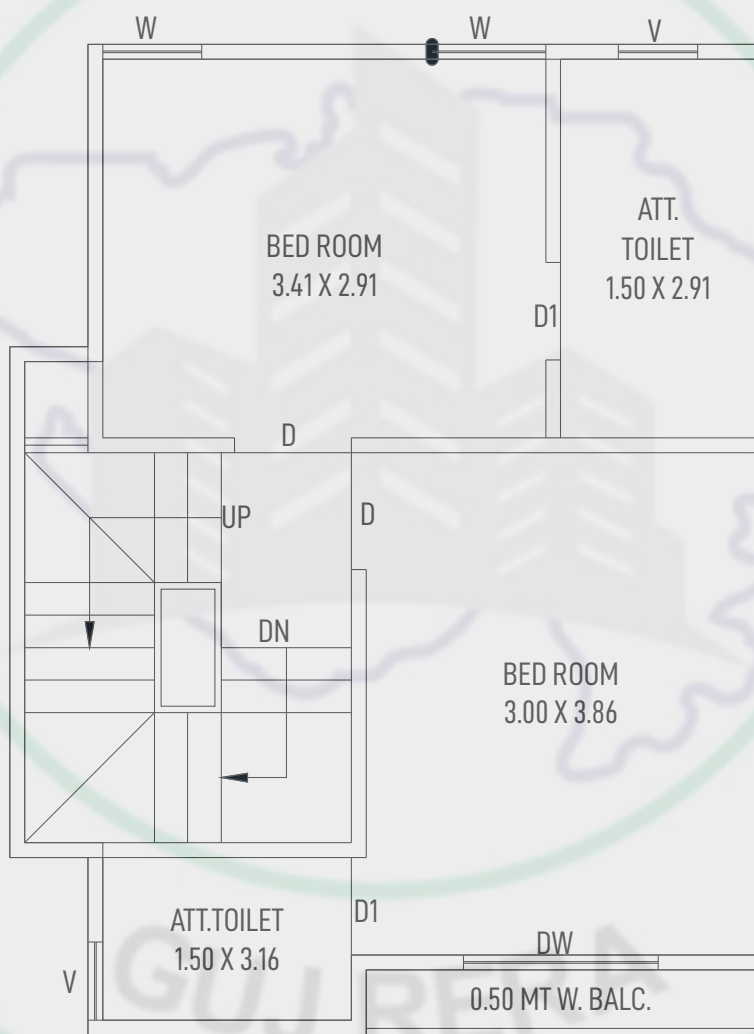
FIRST FLOOR PLAN (TYPE-B)
