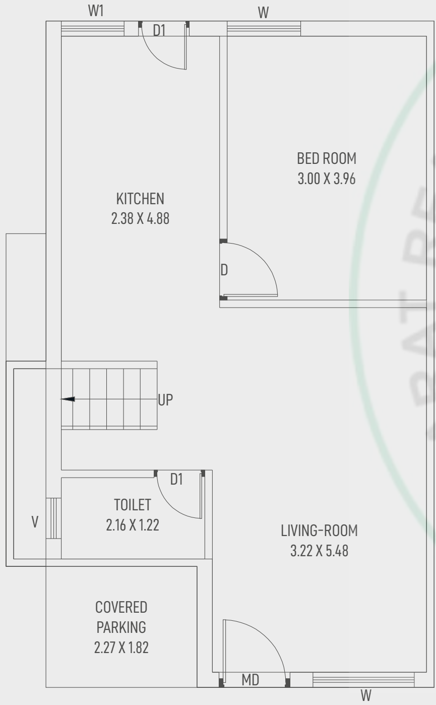
GROUND FLOOR PLAN (TYPE-C)
