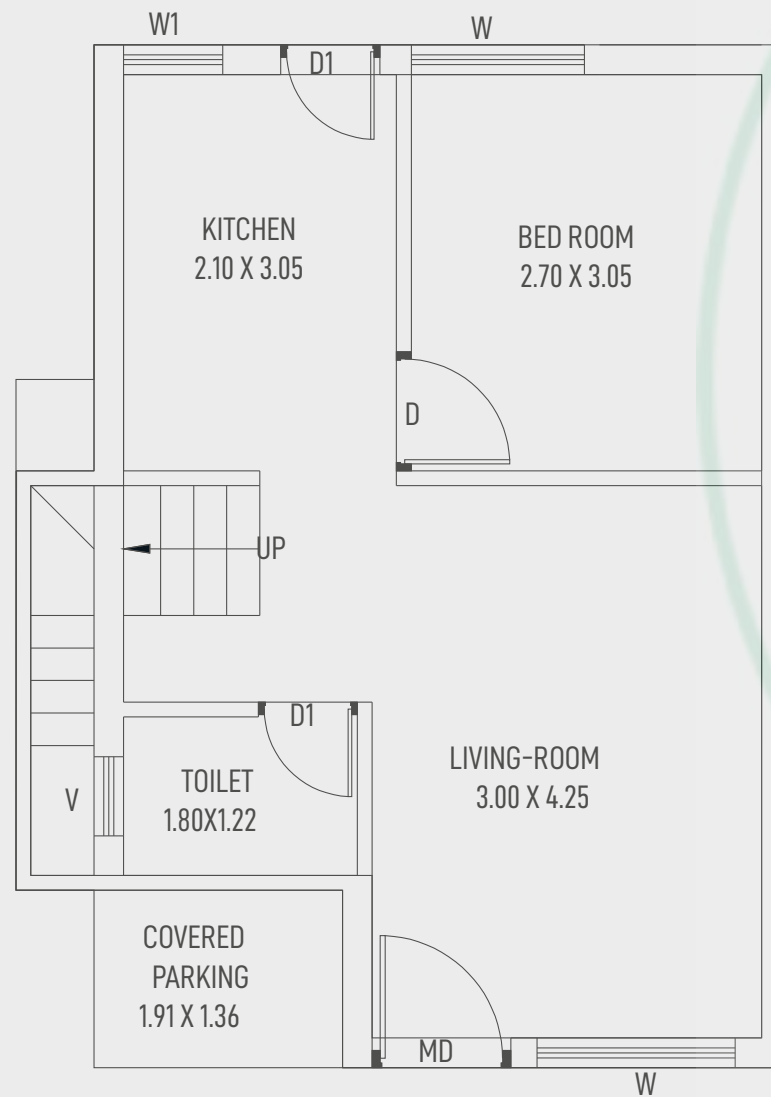
GROUND FLOOR PLAN (TYPE-D)
