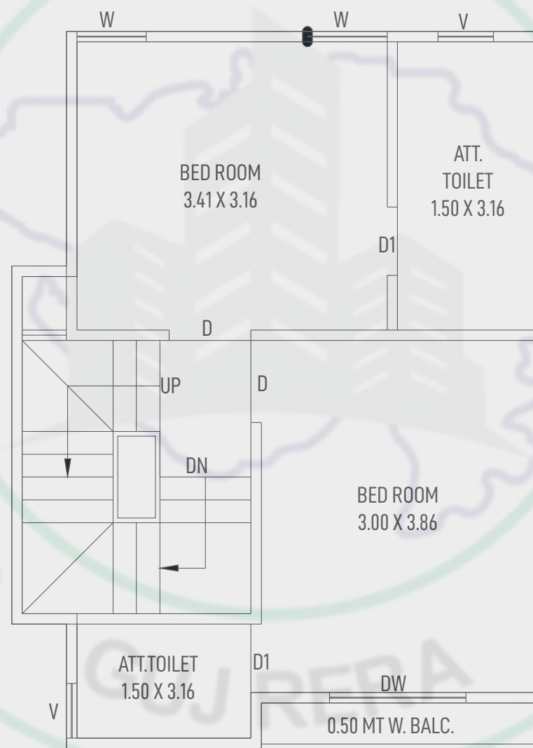
FIRST FLOOR PLAN (TYPE-D)
