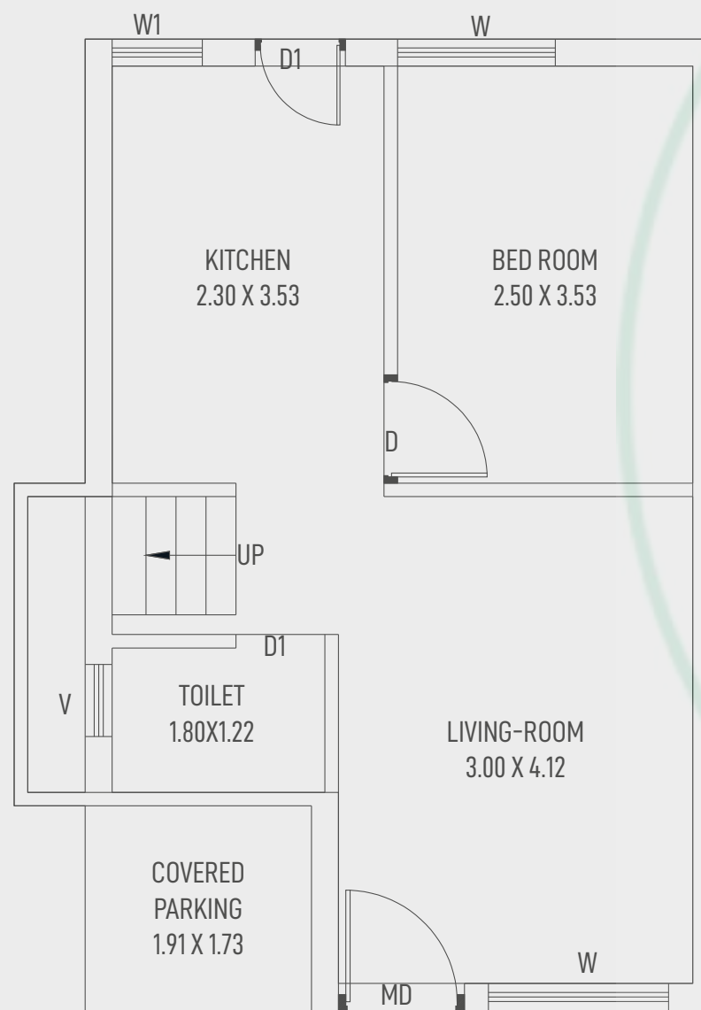
GROUND FLOOR PLAN (TYPE-B1)
