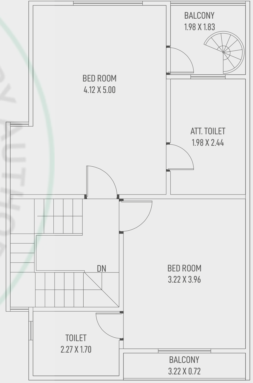
SECOND FLOOR PLAN (TYPE-C)
