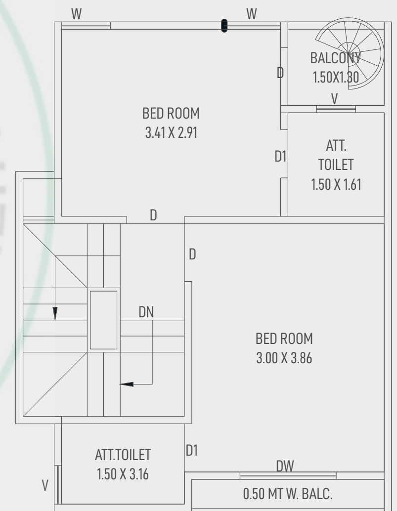
SECOND FLOOR PLAN (TYPE-B)
