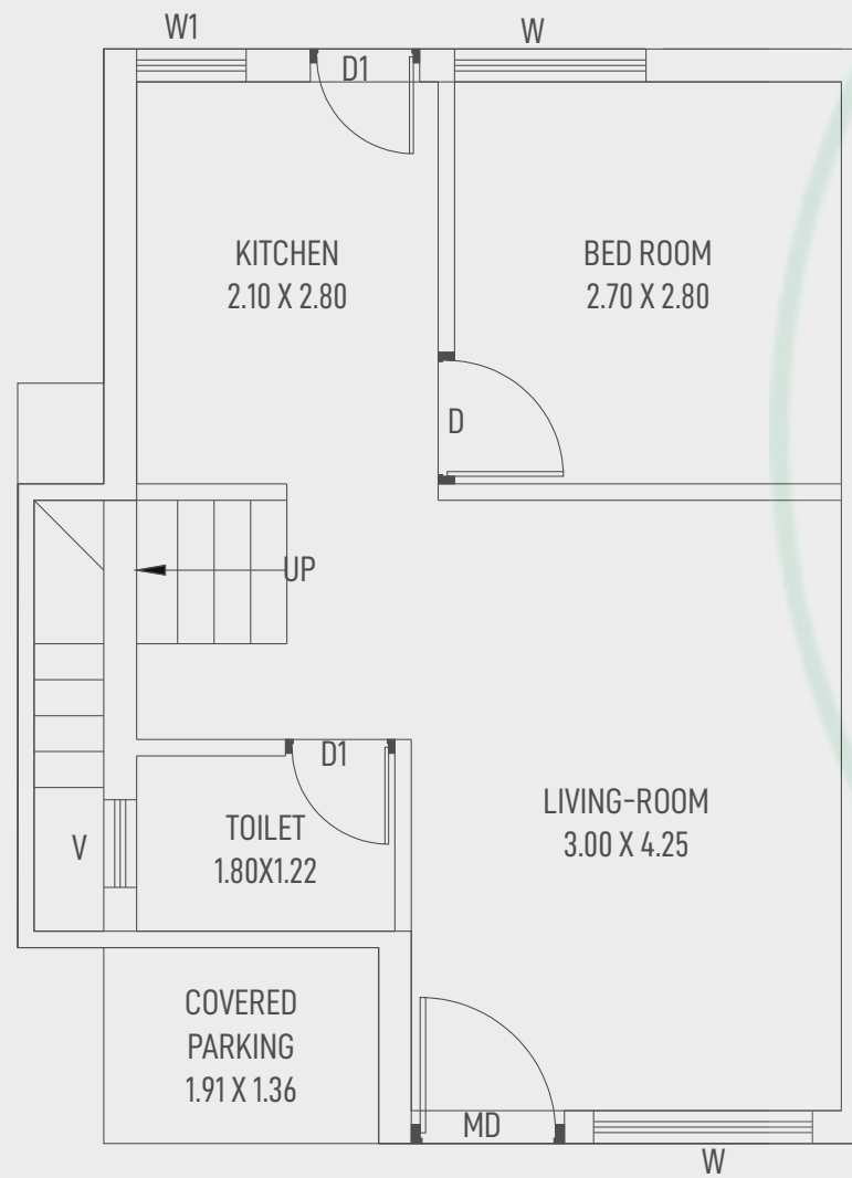
GROUND FLOOR PLAN (TYPE-B)
