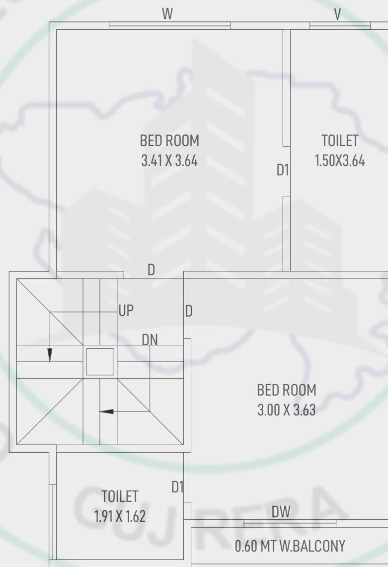
FIRST FLOOR PLAN (TYPE-B1)
