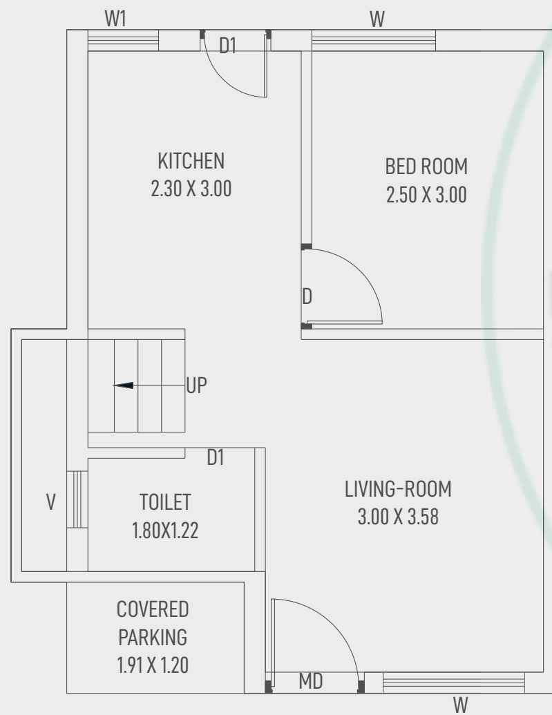
GROUND FLOOR PLAN (TYPE-B2)
