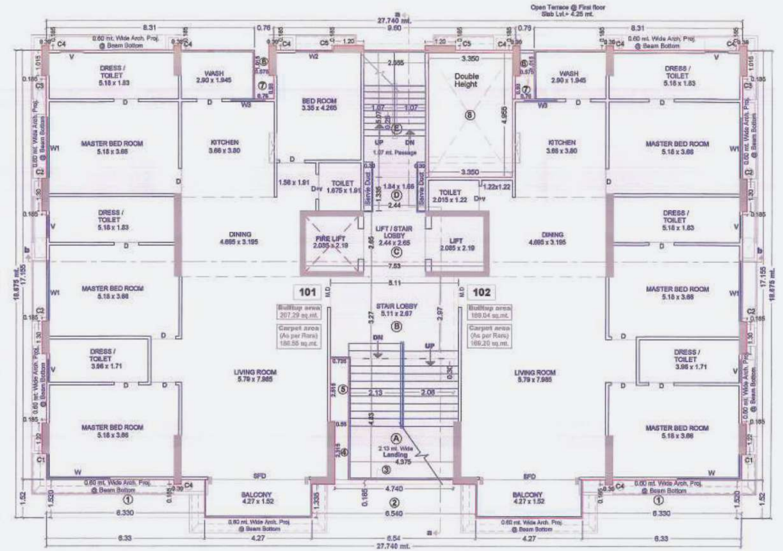
FIRST FLOOR PLAN Lvl. + 4.30 mt.
