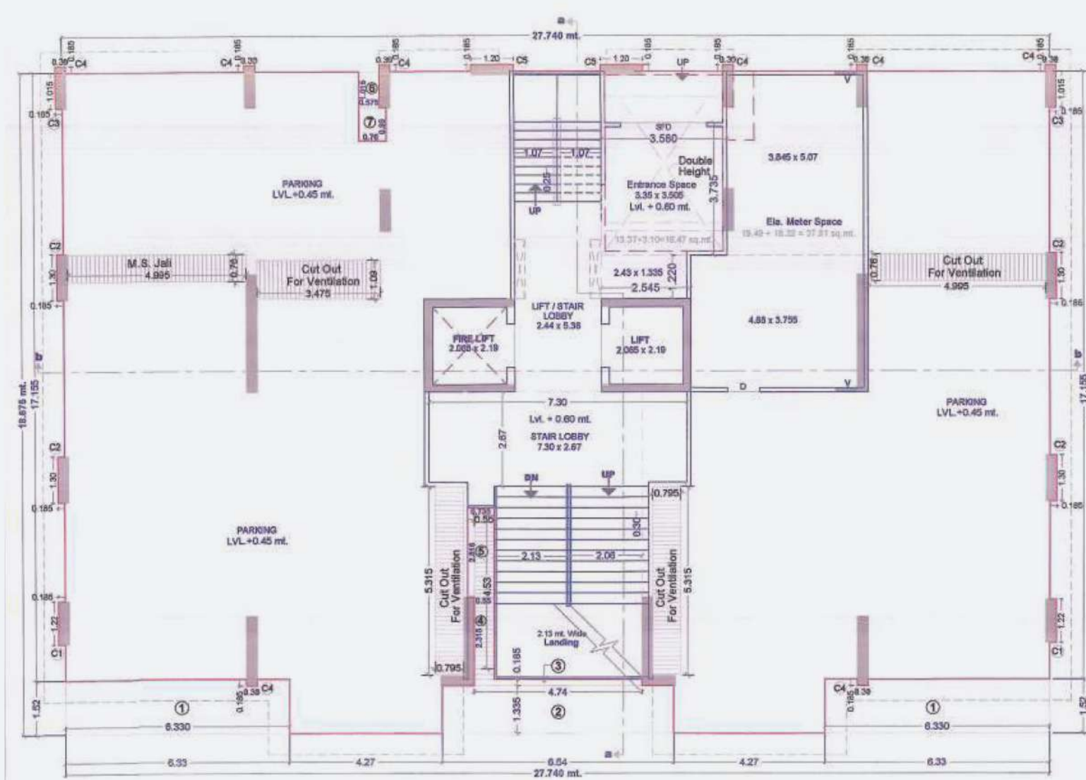
GROUND FLOOR PLAN Lvl. + 0.45 mt.
