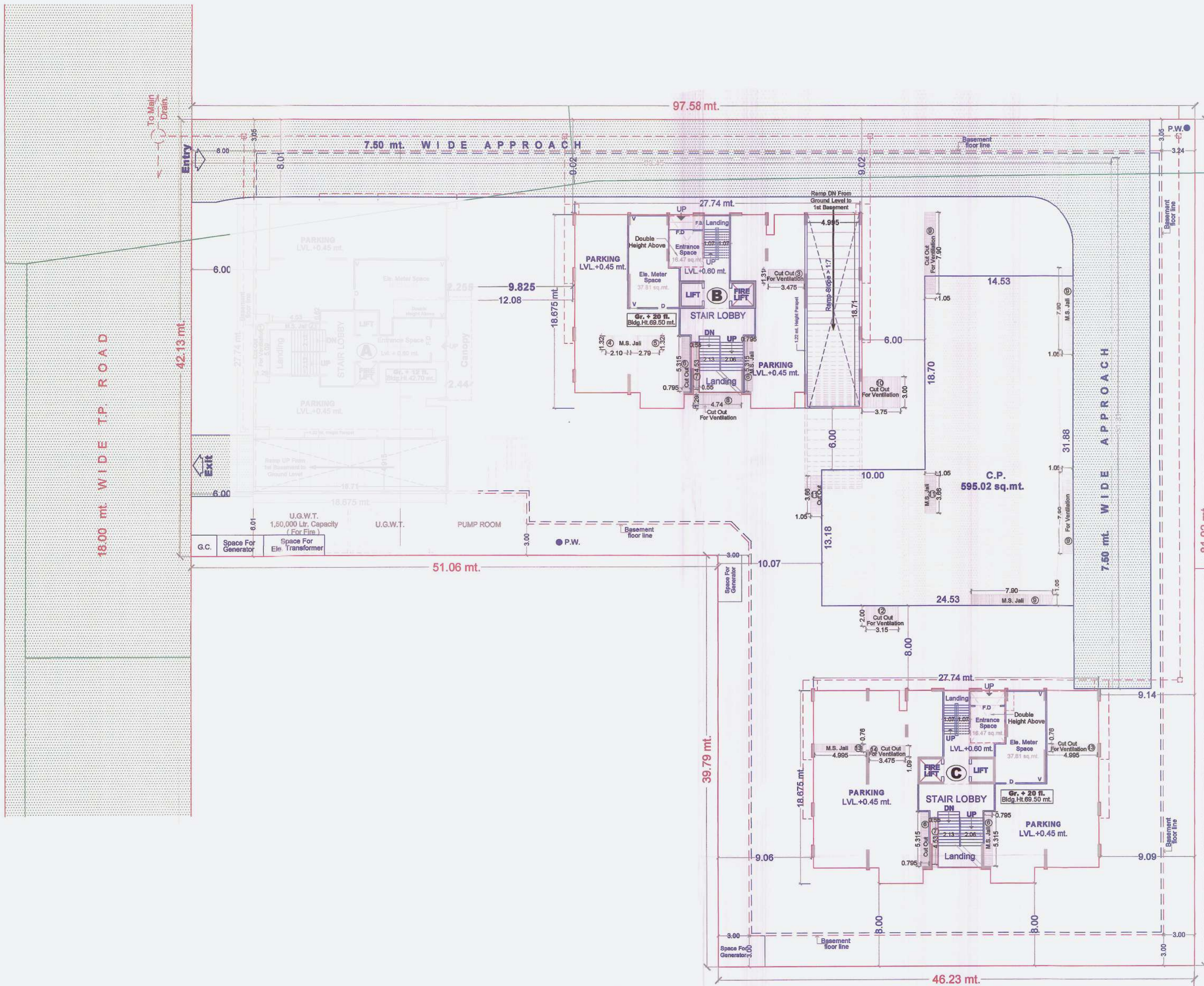
GROUND FLOOR LAYOUT PLAN
