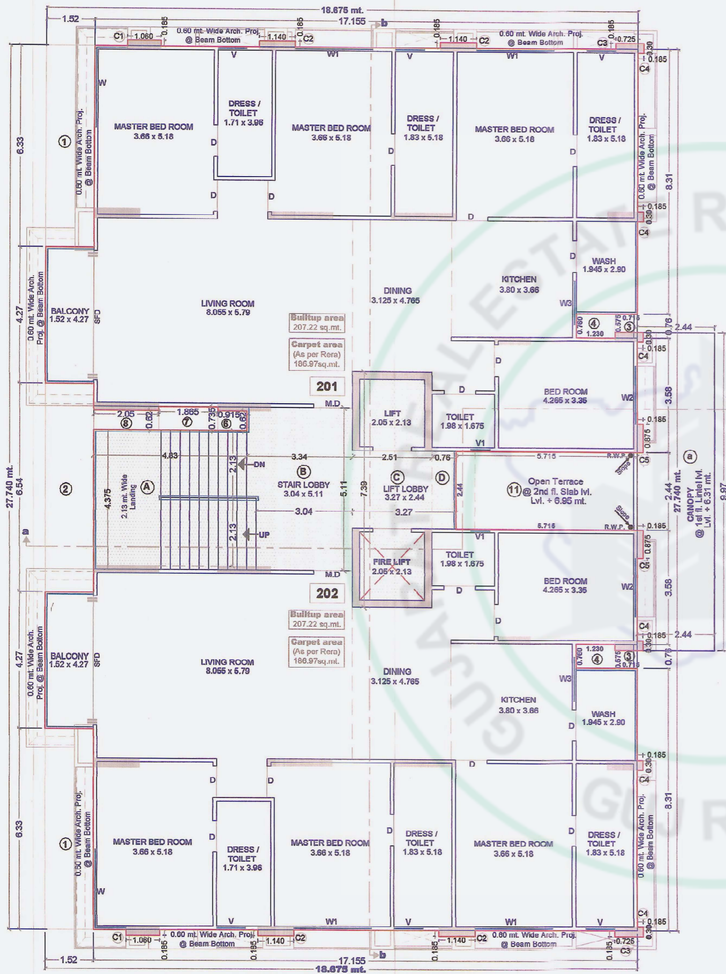
TYPICAL FLOOR PLAN (2nd. to 12th. Floor) Lvl. + 6.95 mt. To Lvl. + 39.42 mt.
