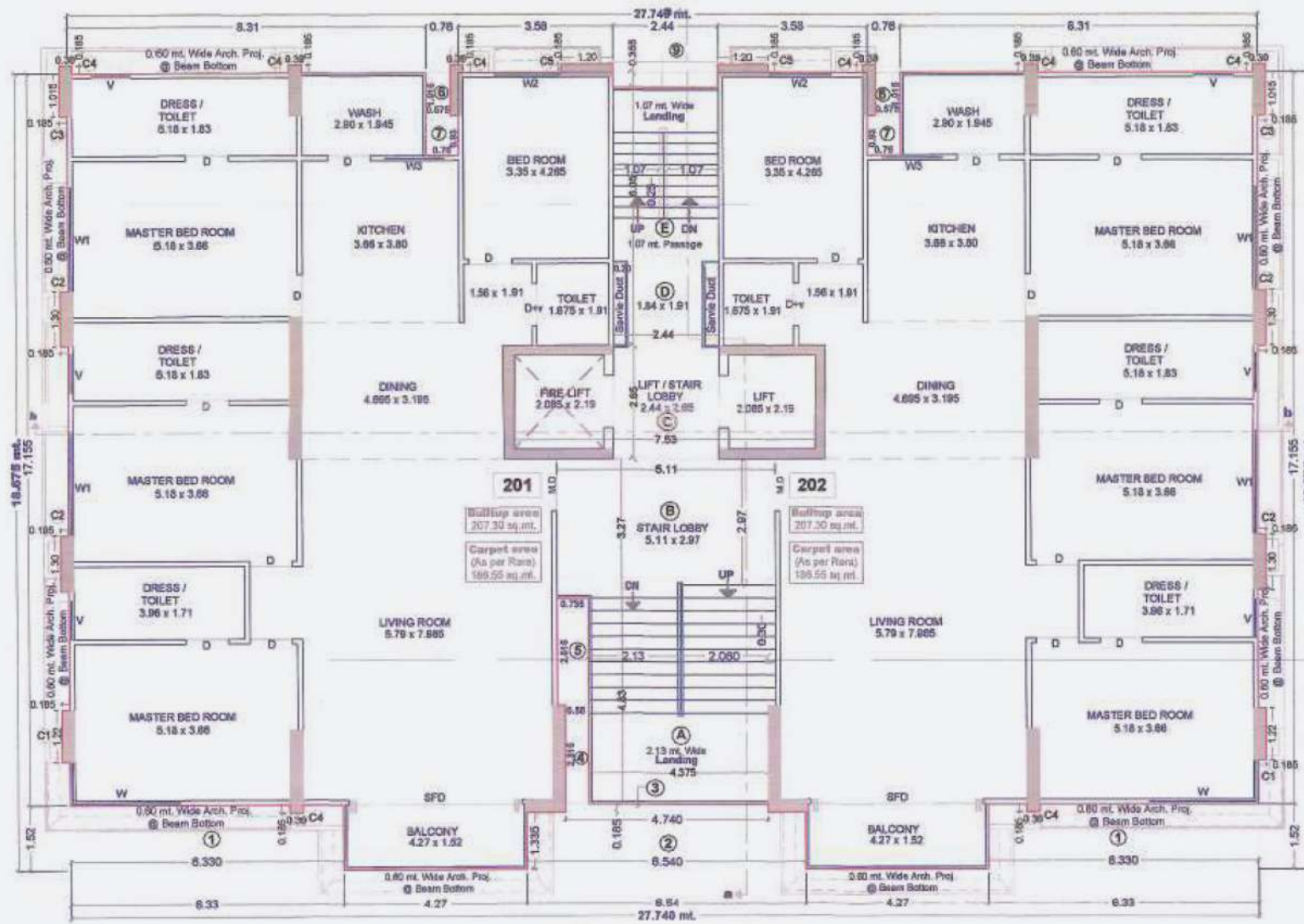
TYPICAL FLOOR PLAN (2nd. to 20th. Floor) Lvl. + 7.56 mt. To Lvl. + 66.24 mt.
