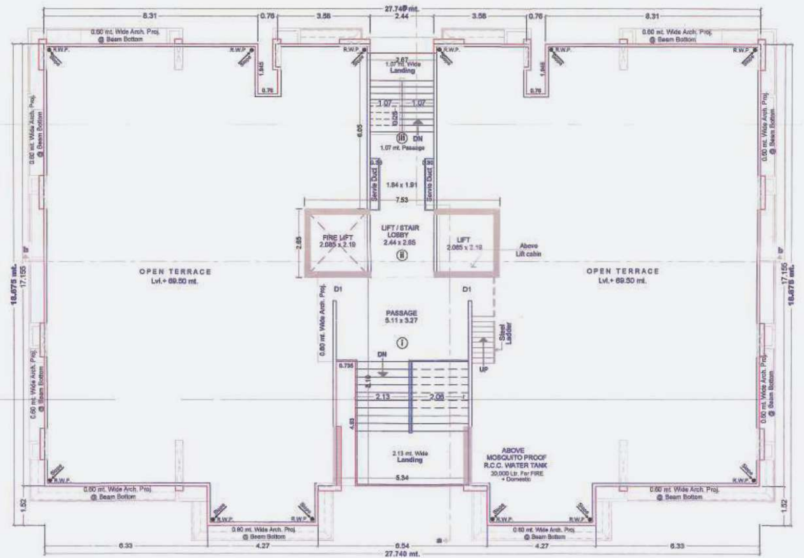
TERRACE FLOOR PLAN Lvl. + 66.50 mt.
