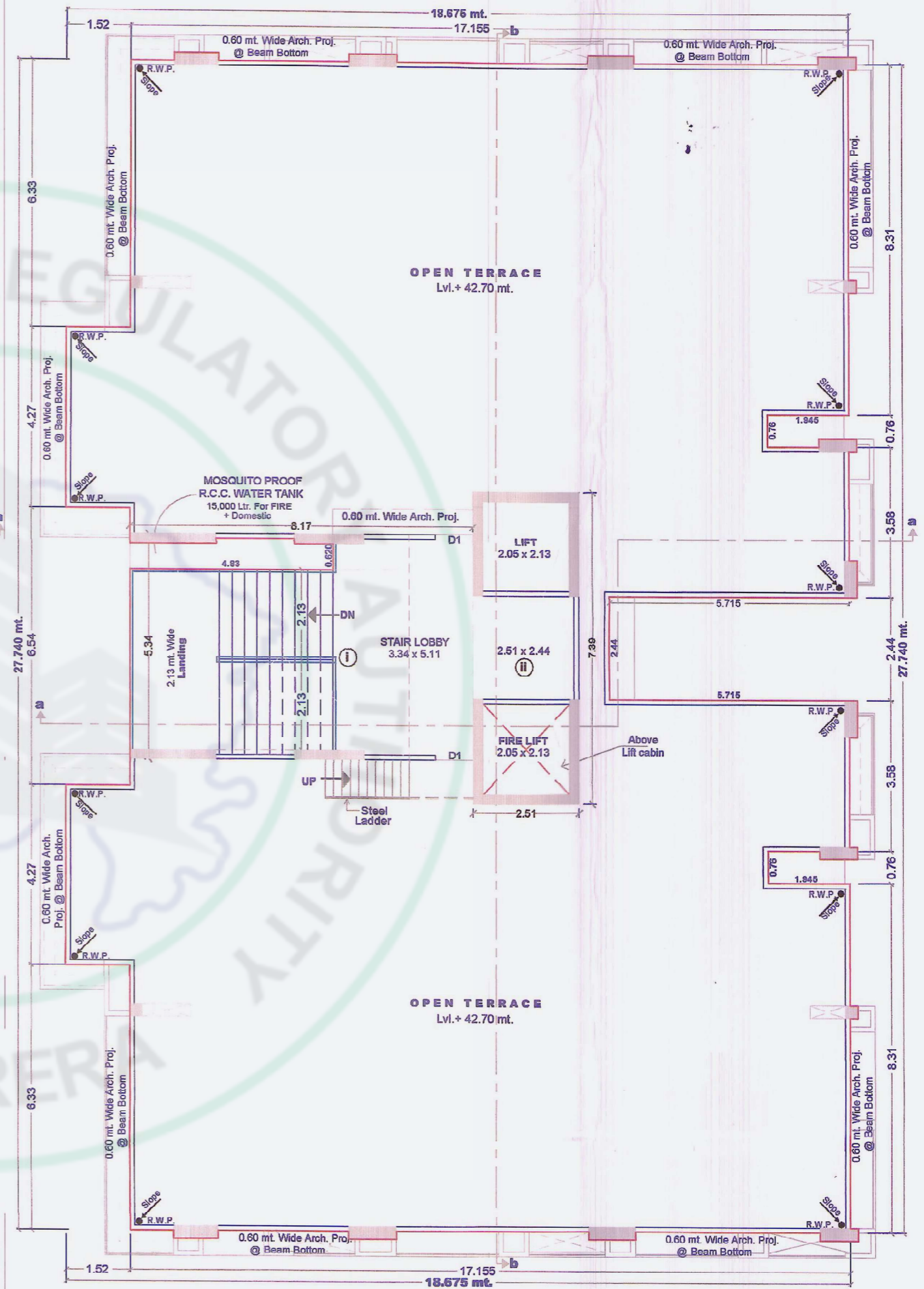
TERRACE FLOOR PLAN Lvl. + 42.70 mt.
