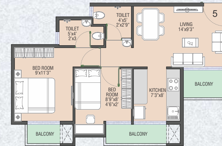
2 BHK | UNIT PLAN
