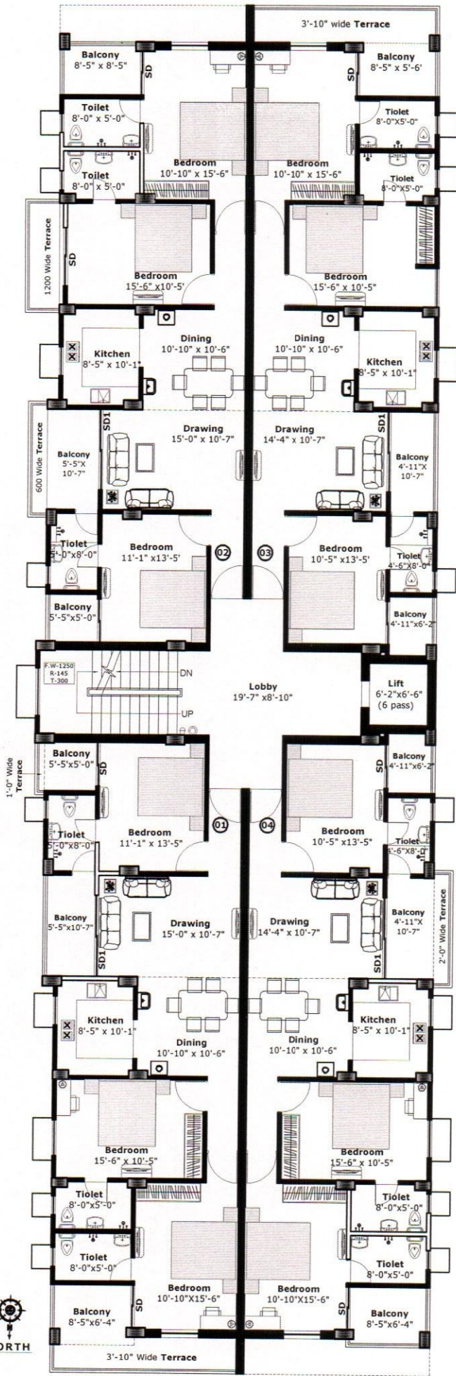
Typ. 2nd & 4th FLOOR (BOOKING) PLAN.
