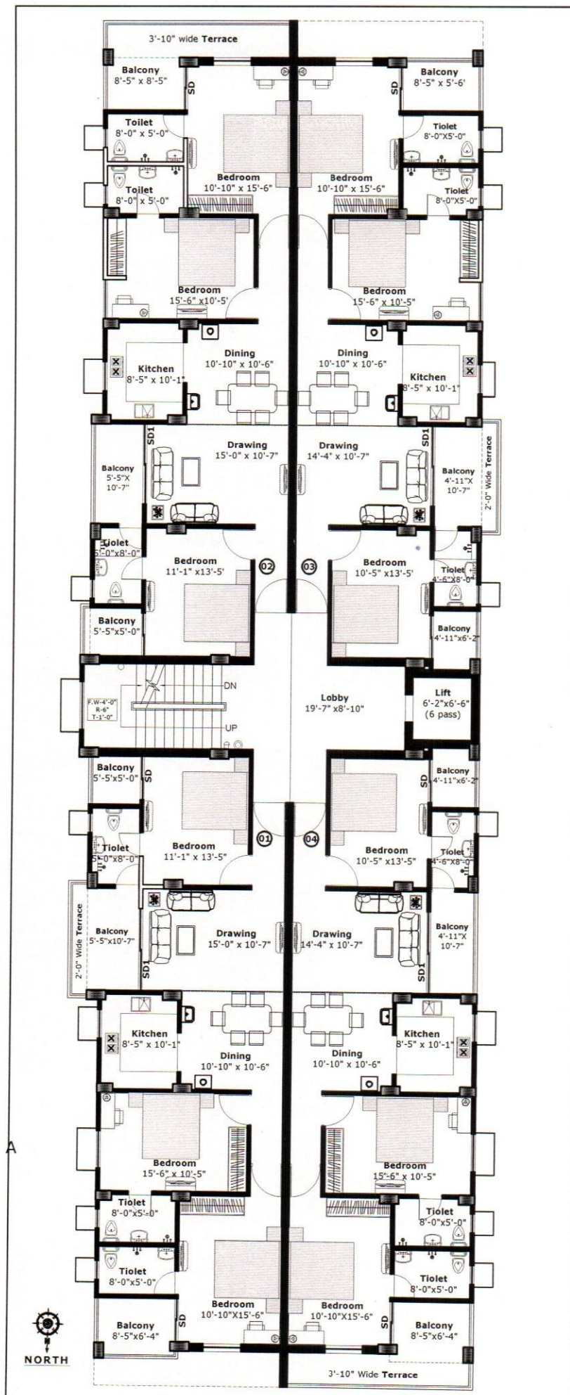
TYP. 1st & 3rd FLOOR (BOOKING) PLAN.
