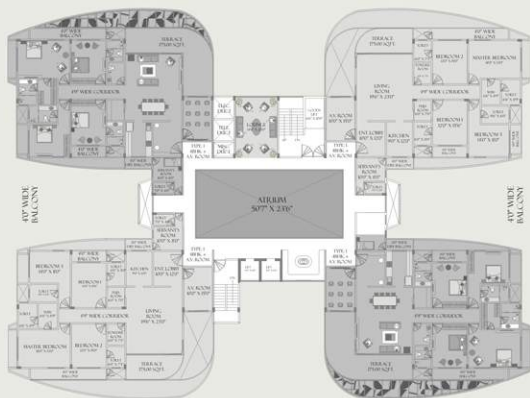
TYPICAL PLAN - 1ST, 3RD, 5TH, 7TH FLOOR
